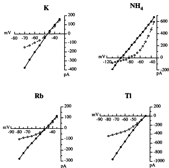
FIGURE 2 Current-voltage relationships for the cell illustrated in Fig. 1 with each permeating ion. Instantaneous current (●) was measured at the beginning of the voltage step (at time = 100 ms) and steady-state current (○) was measured at the end of the voltage step. Erev is the intersection of the two curves. A second intersection was approached at the holding potential and represents a crossover between deactivation and activation of M-current. Erev in this cell was K = -47 mV; NH 4 = -100 mV; Rb = -50 mV; and Tl = -35 mV.
